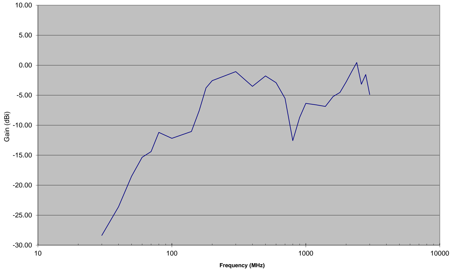
EM-6105-1 Typical Gain
